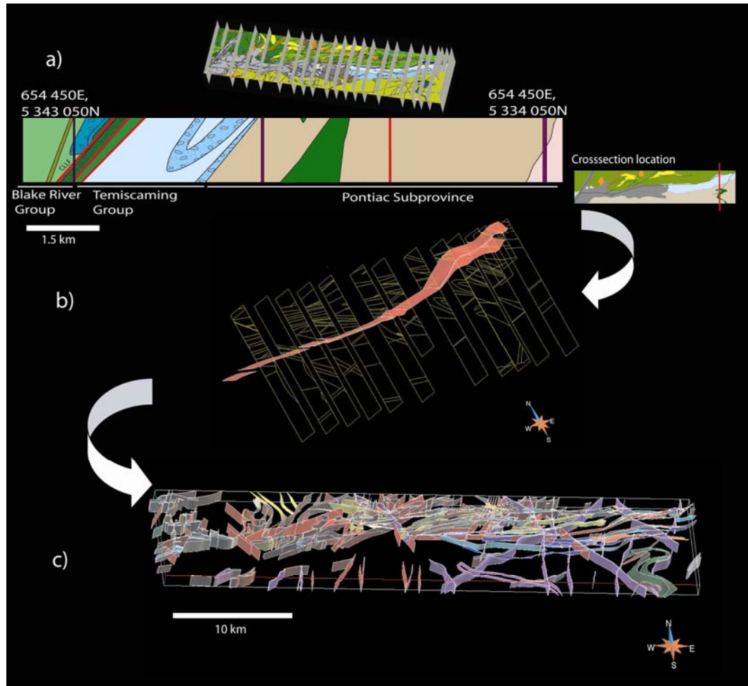
Figure 2-4: a. Location and example of the interpreted cross sections; b. Surface representation of the CLLF being constructed by joining the dip interpretations in each cross section; c. Surface model of the study area (without the Proterozoic sedimentary cover and Archean units underneath).
