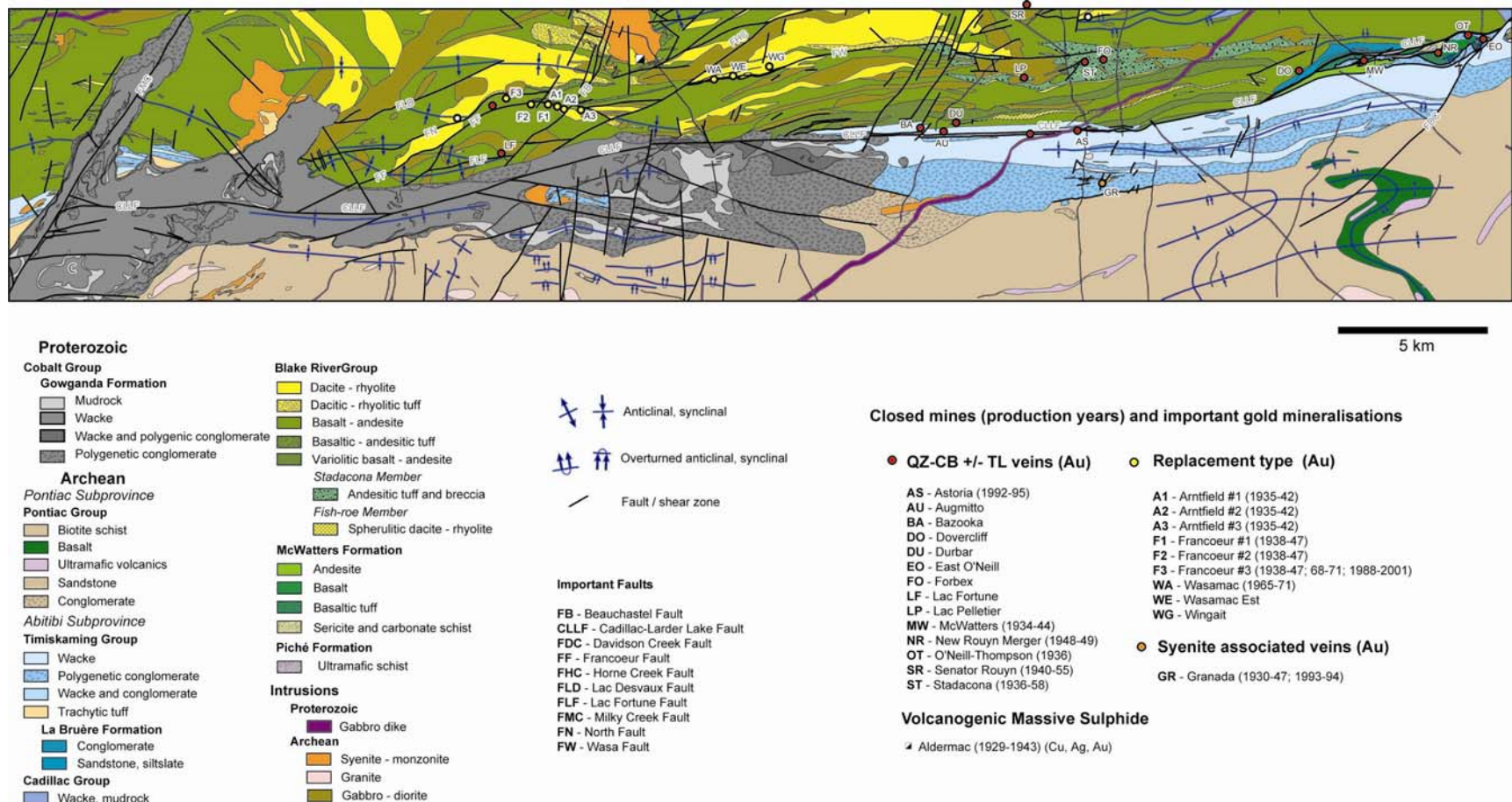
Figure 2-2: Geological map of the study area with location of mines and mineral deposits (modified from Legault and Rabeau, 2007)
