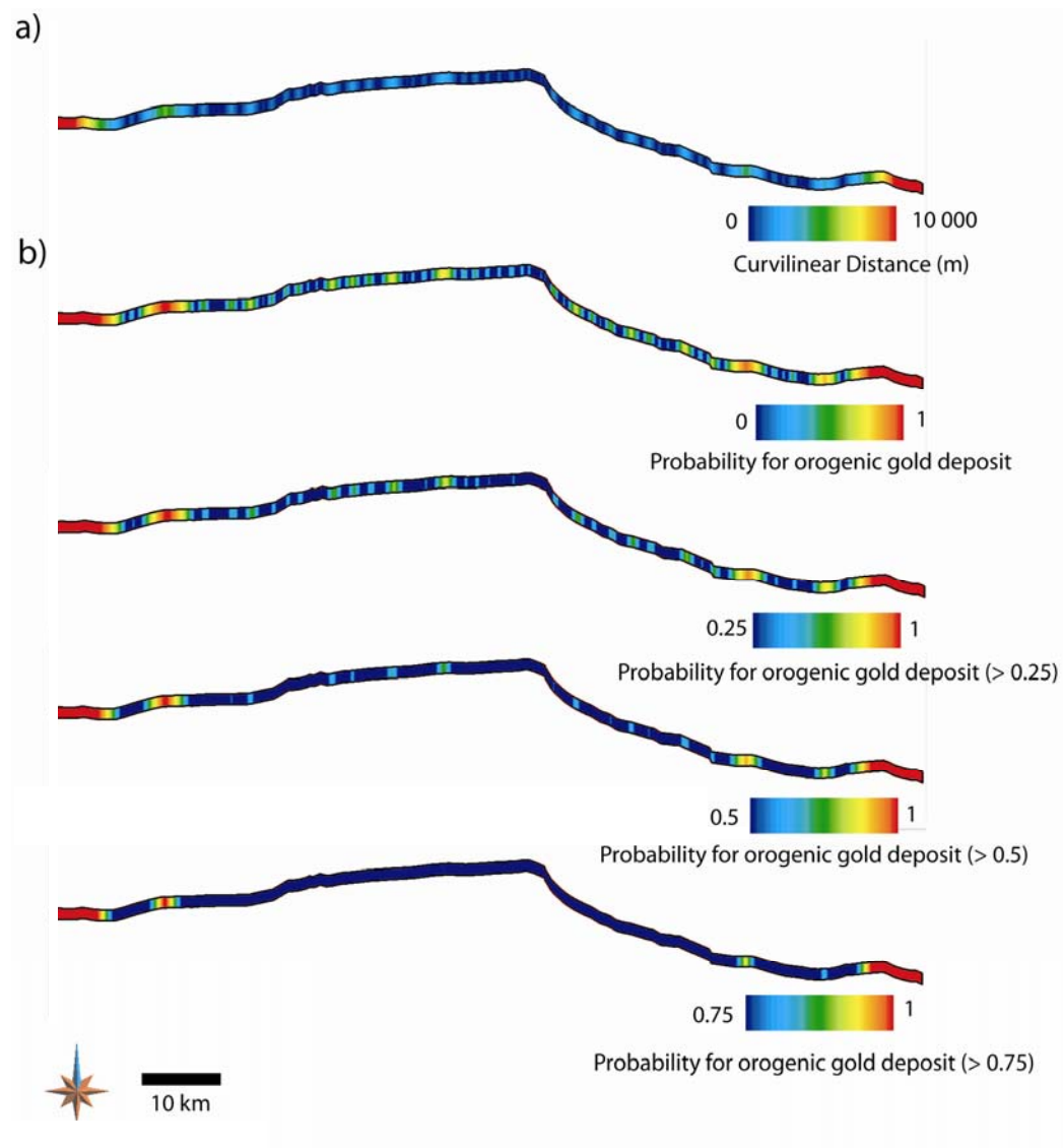
Figure 1-6: a) Curvilinear inter distance between known orogenic gold mineralizations mapped on the trace (1 km buffer) of the Cadillac Larder Lake Fault trace. b) Derived probability maps of potentially unrecognized orogenic Au mineralization occurrences for various confident levels varying from 0 to 1.
