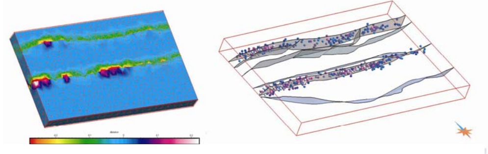
B ) Compression on the Wasa Fault and the CLLF
