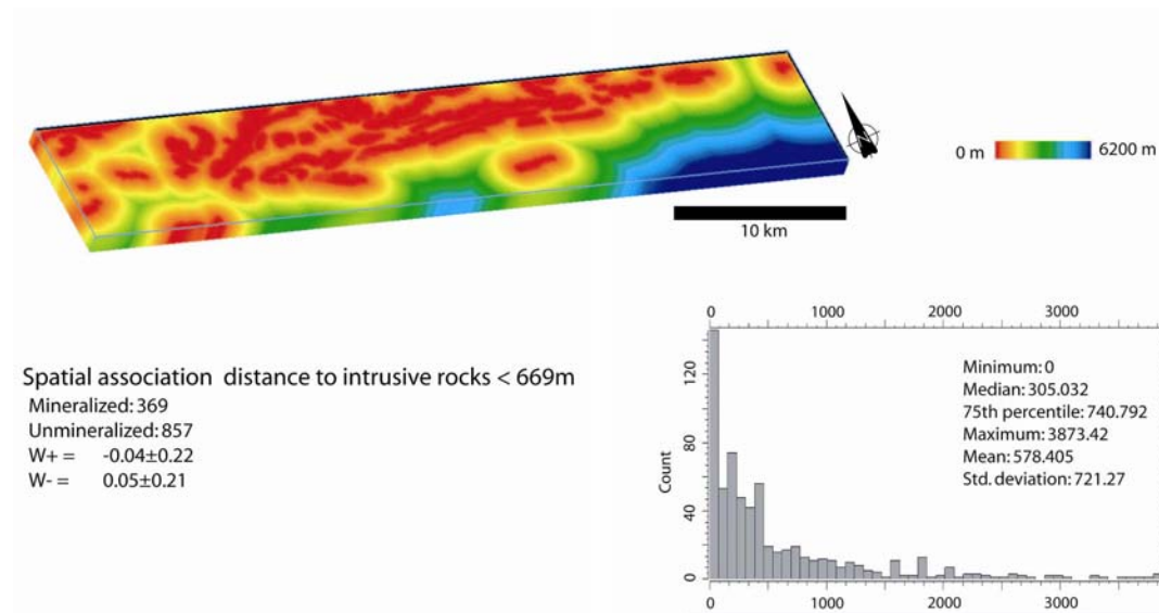
Figure 2-11: Calculated distance to intrusions with accompanying histogram showing the cumulative frequency of mineralized occurrences versus to the distance to the nearest intrusion, with calculated weights and confidence intervals.
