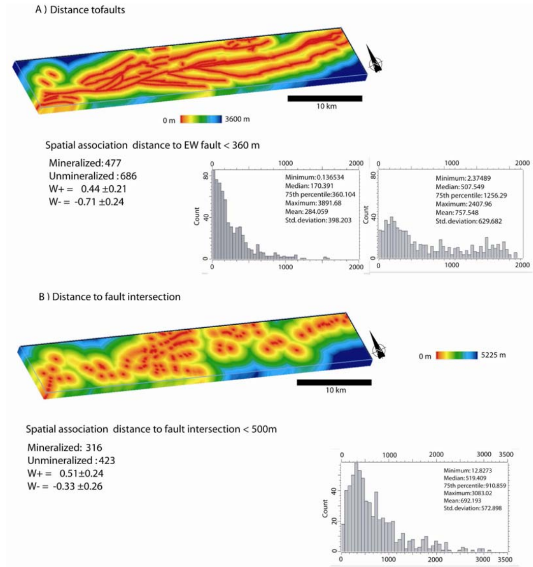
Figure 2-10: Calculated distance of mineralized occurrences to E-W faults (a) and to fault intersections (b). Histograms show the cumulative frequency of mineralized occurrences versus to the distance to both fault groups, and calculated weights with confidence intervals.
