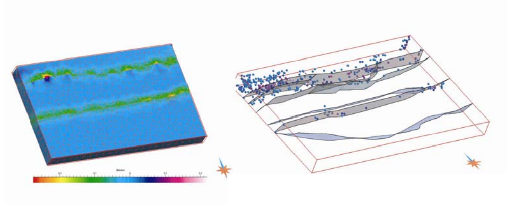
B ) Compression on the Wasa Fault and the CLLF
