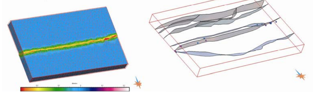
C ) Dextral slip on the CLLF
