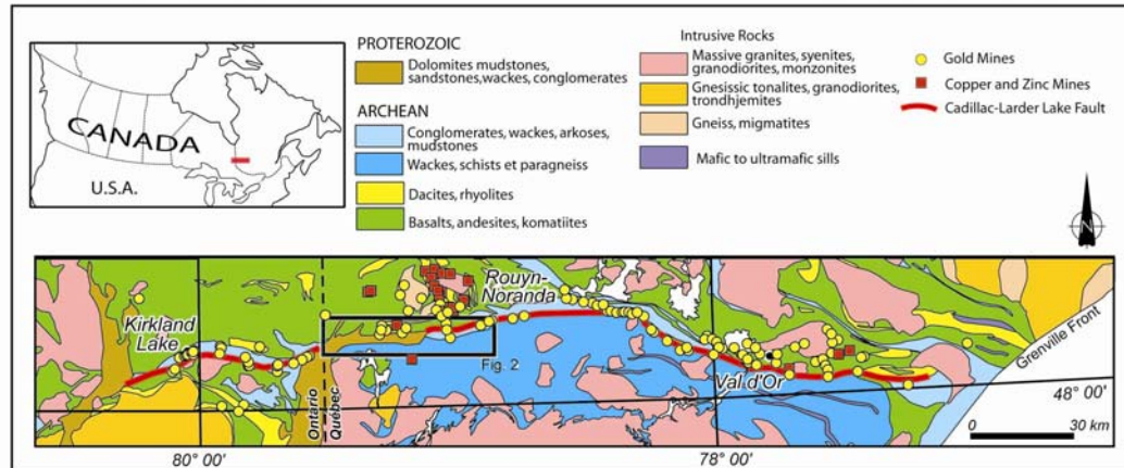
Figure 2-1: Simplified geological map along the Cadillac-Larder Lake Fault (CLLF) showing the location of past and present gold, copper and zinc mines.
