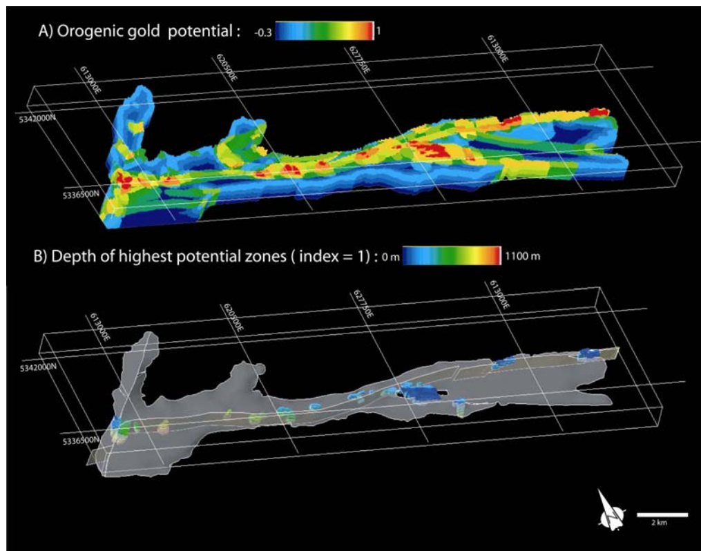
Figure 2-12: a. Mineral potential map for orogenic gold mineralization under the Proterozoic sedimentary cover. Index values vary from -0.3 to 1. b. Location in 3D
