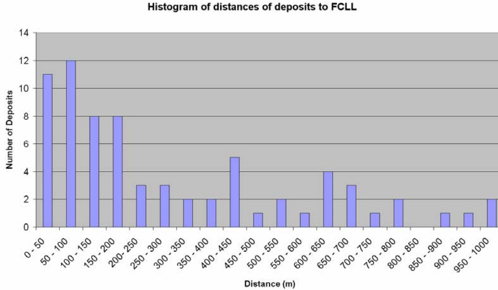
Figure 1-3: Distance of deposits to the Cadillac-Larder-Lake Fault
